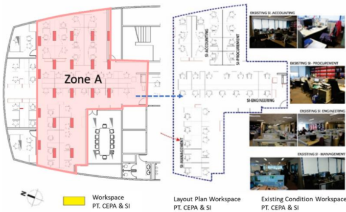
3 Fig. 13: The results of the measurement of workspace Zone A
