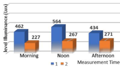
Fig. 6: Linear and bar graphs on illuminance values in workspace (Room 2)
