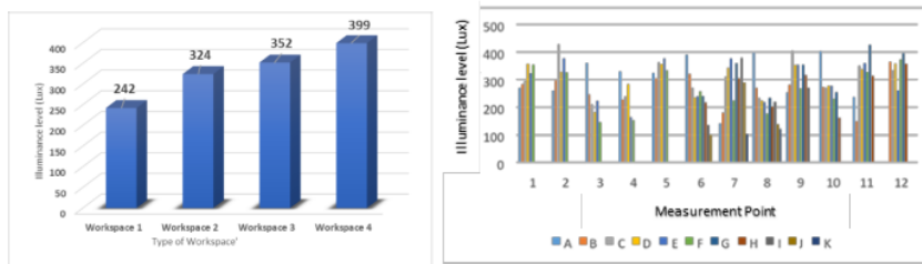
3 Fig. 14: The results of the measurement of light intensity in the work area (Zone A)
